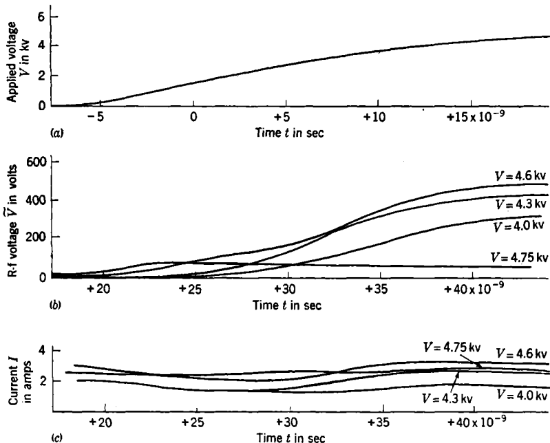
FIG. 8-40.—The buildup of magnetron current and r-f voltage through the operating range of applied voltage. (a) Typical applied voltage; (b) envelopes of r-f oscillations for different applied voltages; (c) tube currents for different applied voltages. (The ordinate is the voltage developed at the oscillograph, and is proportional to the r-f voltage within the magnetron.)
